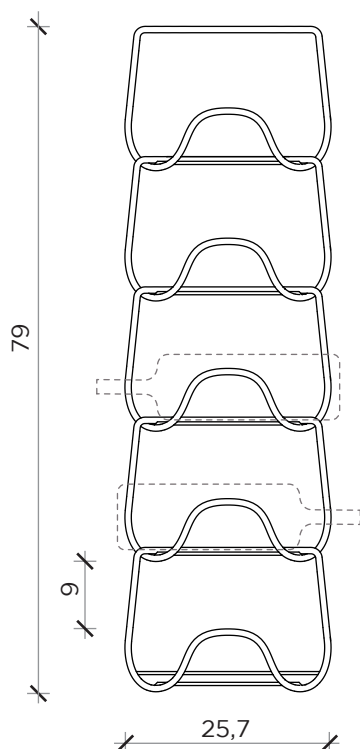
FRONTE | FRONT
