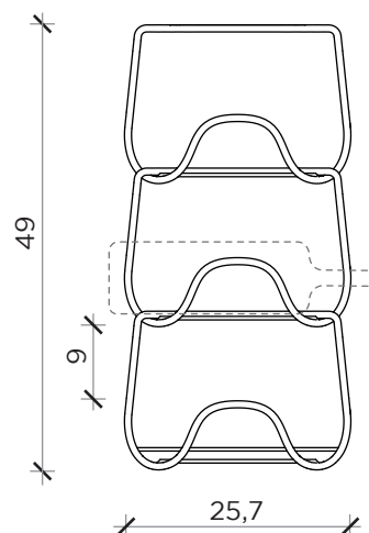
FRONTE | FRONT
